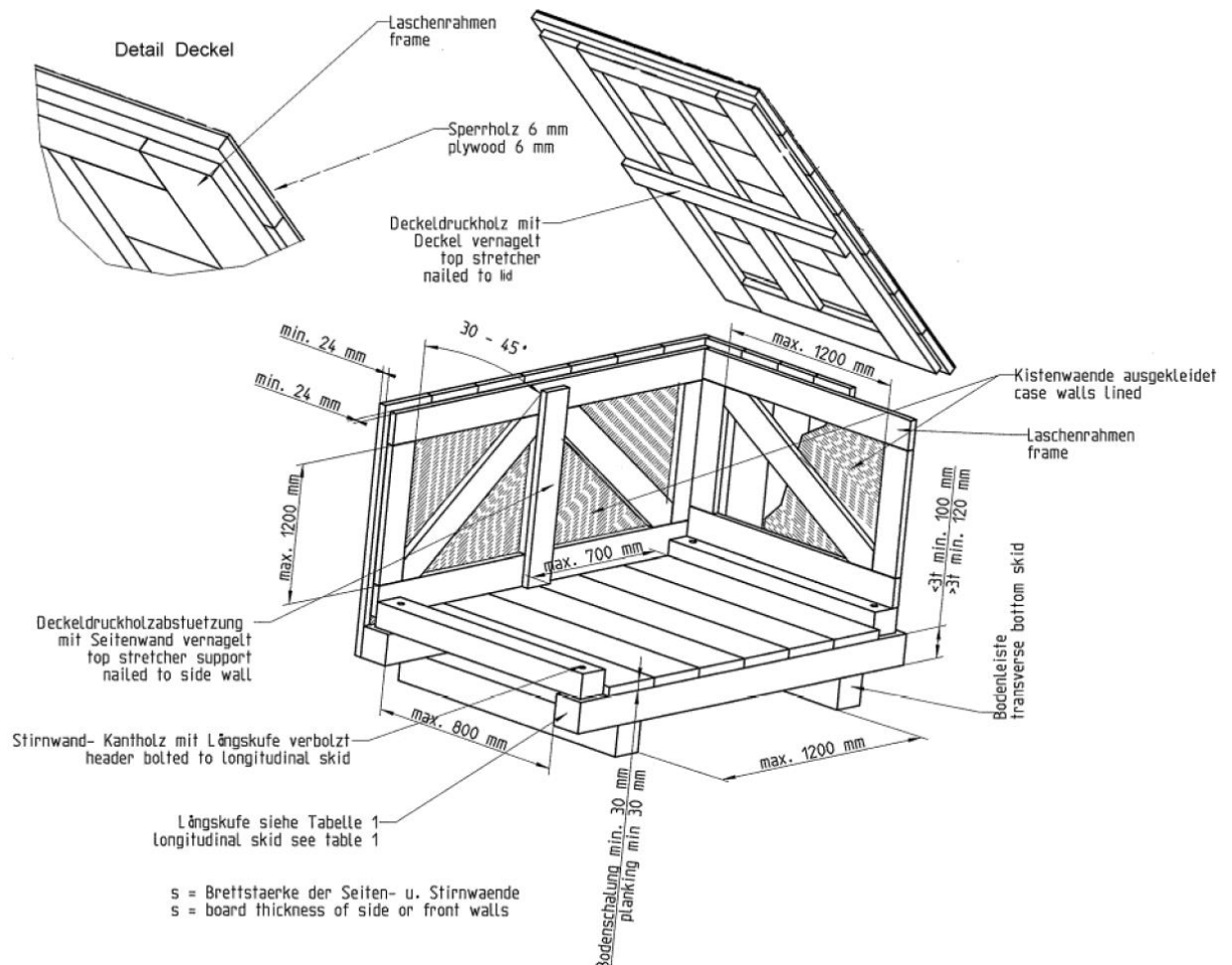
Figure 2: seaworthy - wooden
